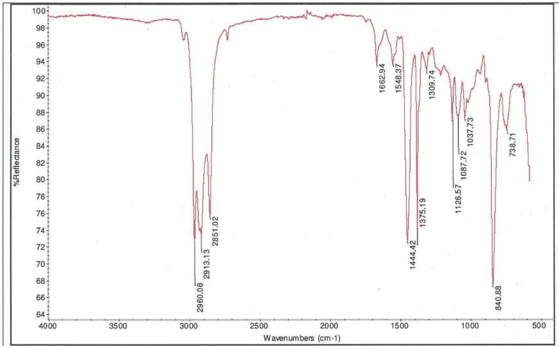
Fig.1: FTIR spectrum of original sample
