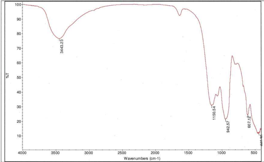
Fig.2: FTIR spectrum of calcination residue
